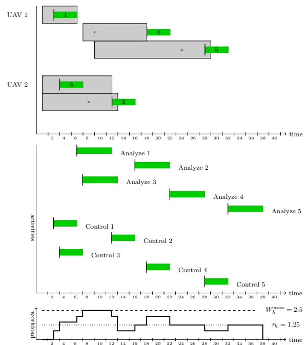
Figure 10: Model E ( W_h^{\max} = 2.5 , \tau_h = 1.25 ).
