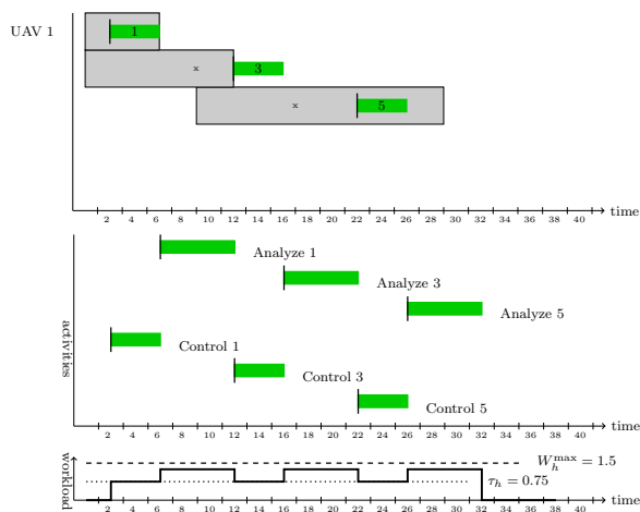
Figure 8: Model C ( W_h^{\max} = 1.5 , \tau_h = 0.75 ).
