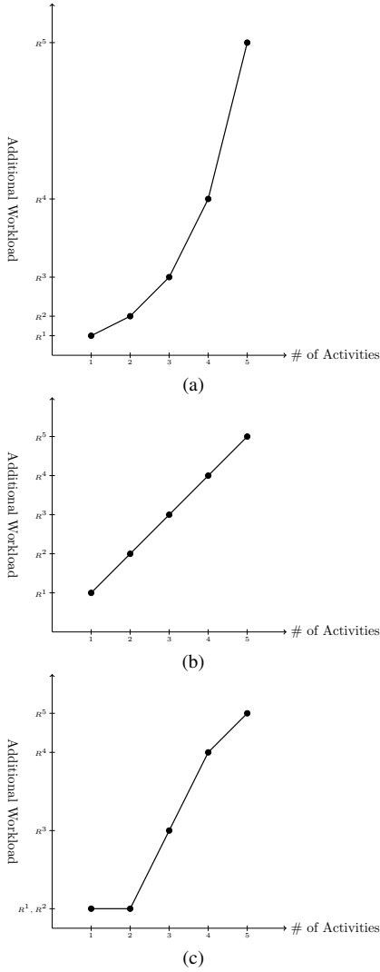
Figure 4: Some possible forms of additional workload.
