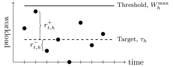
Figure 5: Deviations from the target workload.
