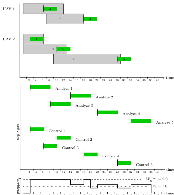
Figure 9: Model D ( W_h^{\max} = 2 , \tau_h = 1.0 ).
