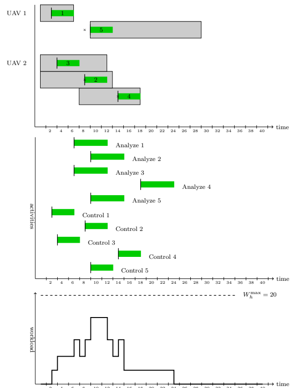
Figure 6: Model A – UAV routes ignore human factors considerations.
