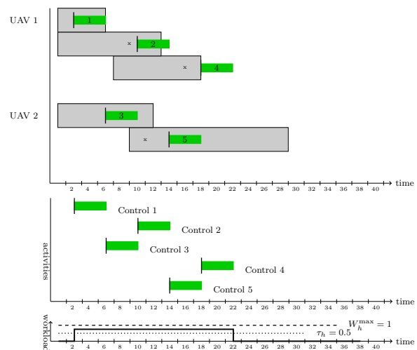
Figure 7: Model B ( W_h^{\max} = 1 , \tau_h = 0.5 ).
