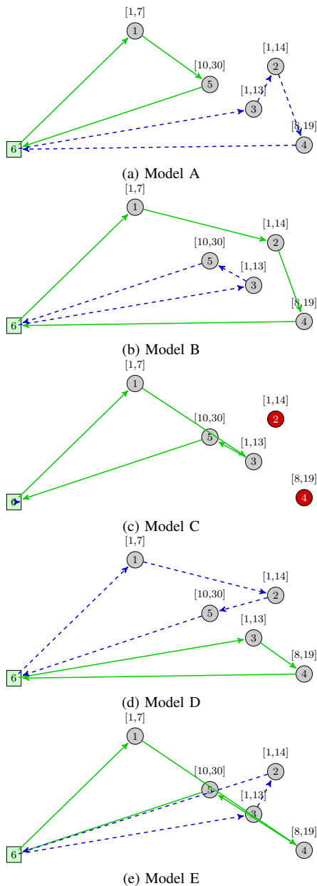
Figure 11: Optimal UAV routes for each model.
