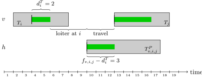
Figure 2: Operator control of UAV traveling between nodes i and j .
